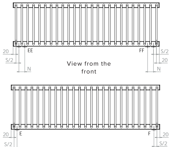
SCE, type 14 and 16 profile
