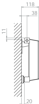
SC single (SCE), type 14 and 16 profile
